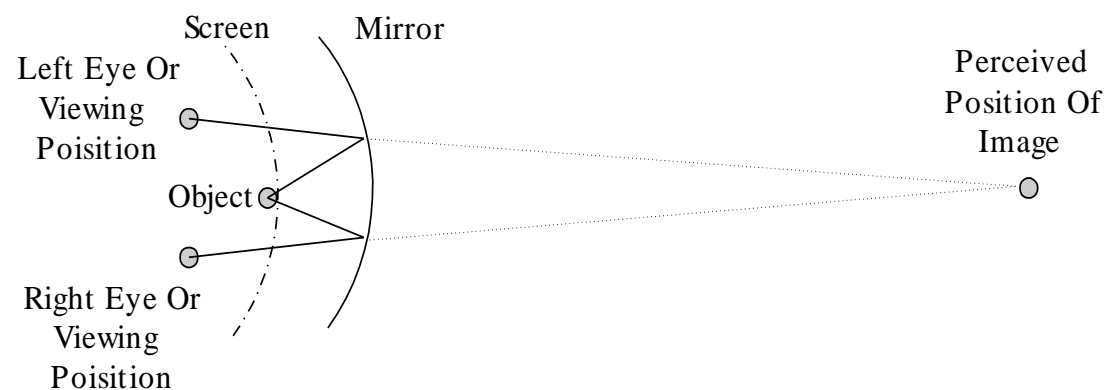
Figure 1: Collimated display
